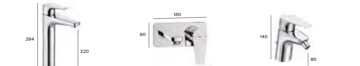
Smooth body extended basin mixer Wall-mounted basin mixer Bidet mixer
